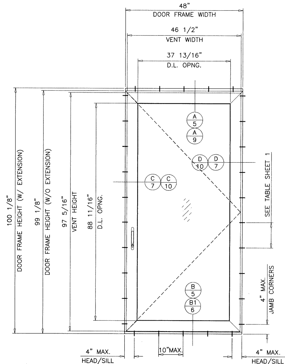
TYPICAL ELEVATION TESTED UNIT
