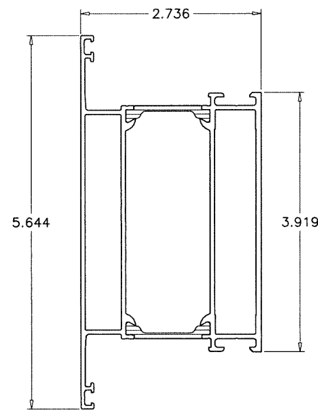
15 WALL ATTACHMENT
