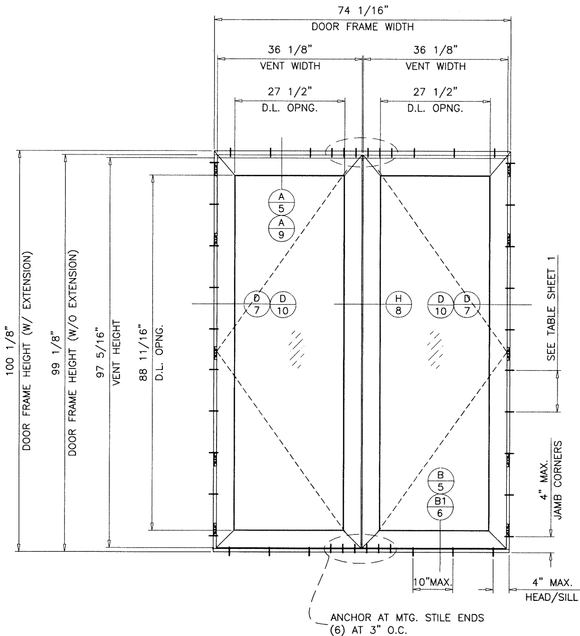
TYPICAL ELEVATION TESTED UNIT
